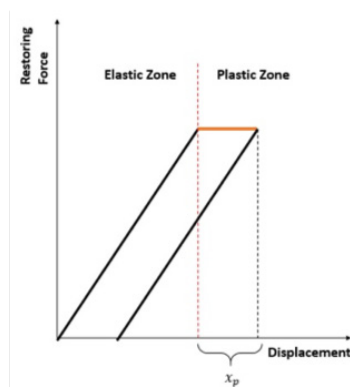
Fig 1. Displacement graph – restoring force
